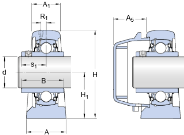
SYFWR 1.3/8 YZTHR Bearing 2D drawings and 3D CAD models
